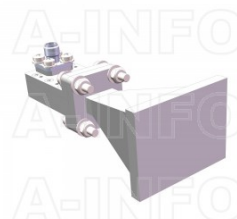
LB-42-15-C-3.5FSPO Standard Gain Horn Antenna 18-26.5GHz 15dB Gain 3.5mm Female
