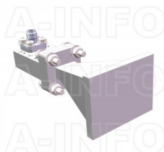
LB-42-15-C-KFSPO Standard Gain Horn Antenna 18-26.5GHz 15dB Gain 2.92mm Female
